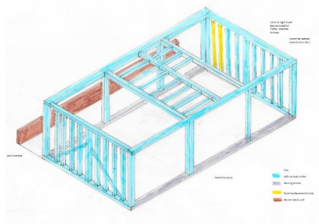
Figure 4 – Isometric drawing showing wall structure
